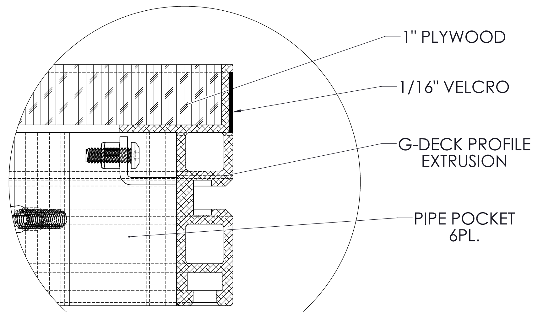
DETAIL B SCALE 1 : 1
