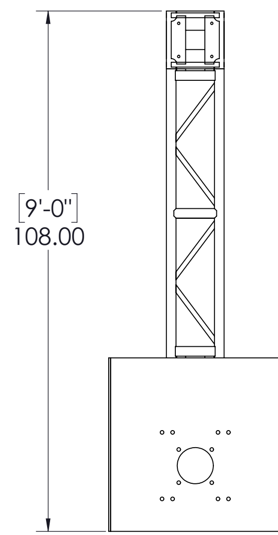
SIDE ELEVATION VIEW
