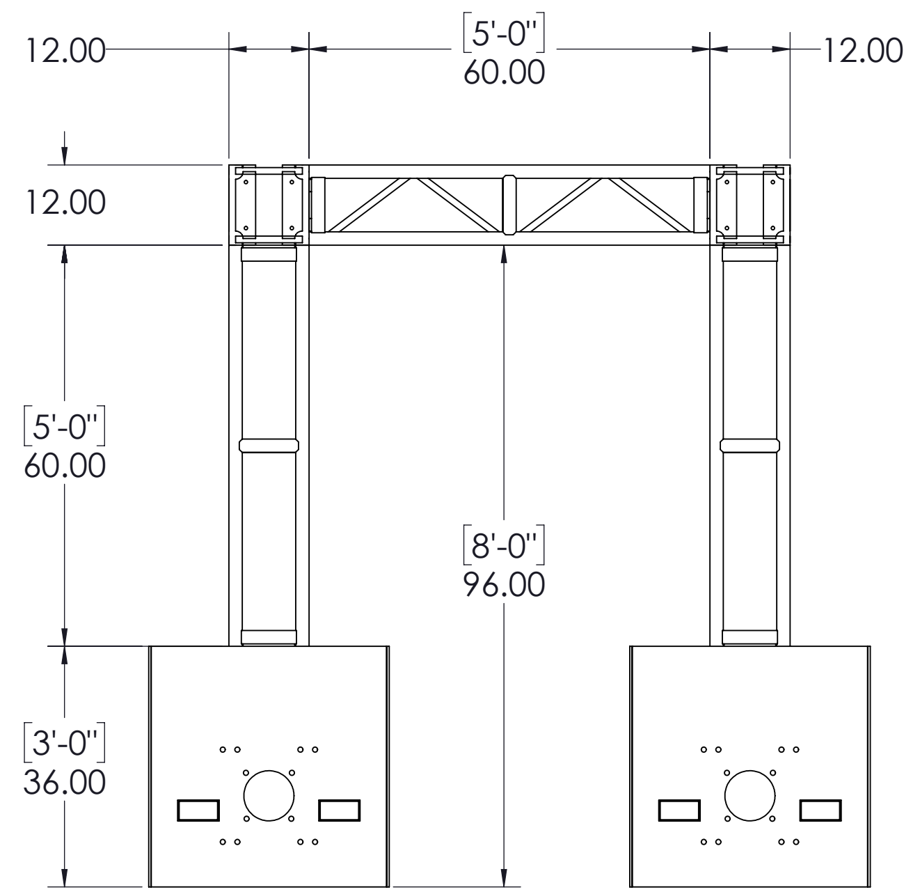
FRONT ELEVATION VIEW
